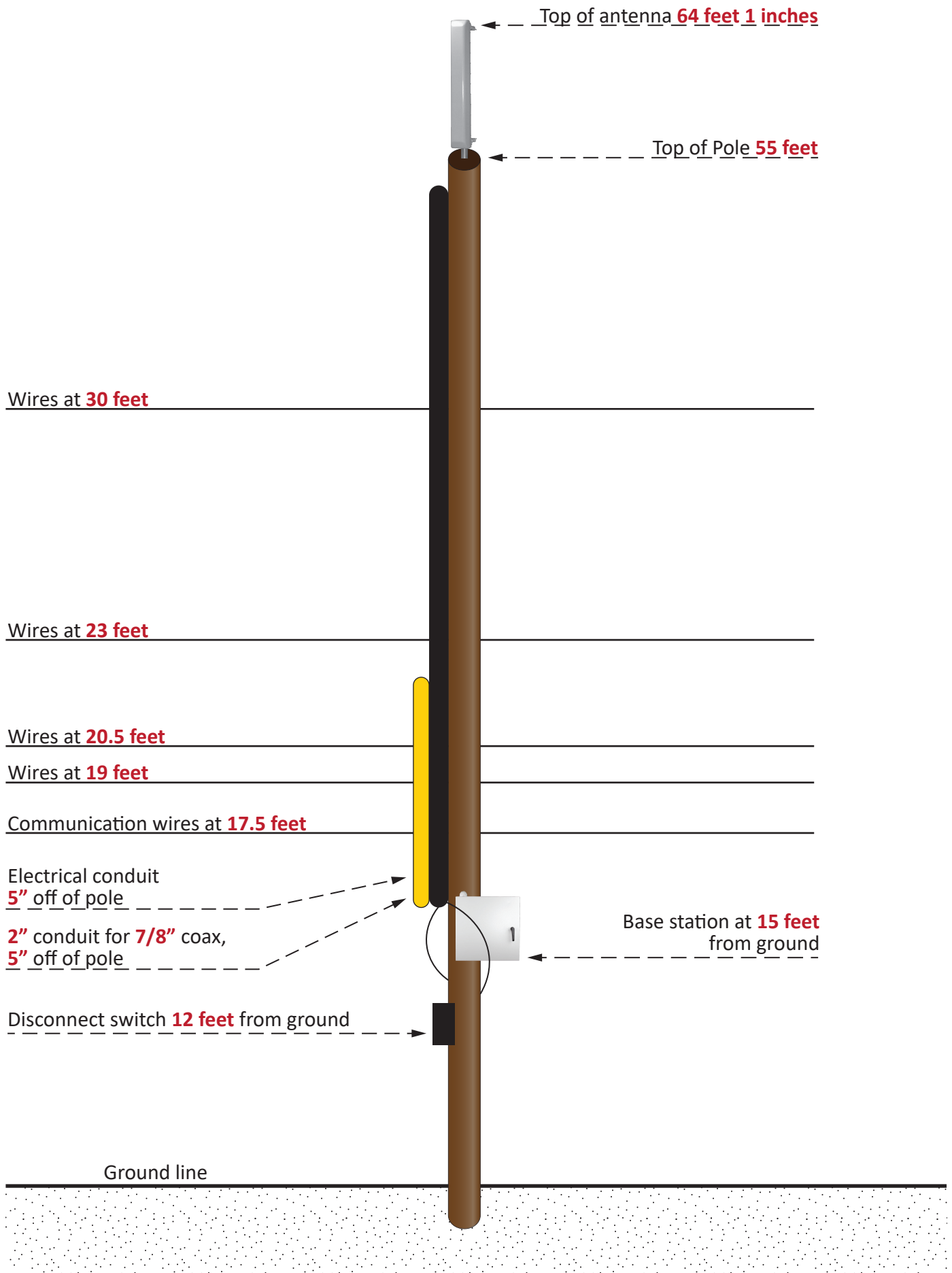
FIGURE 2: POLE DIAGRAM
